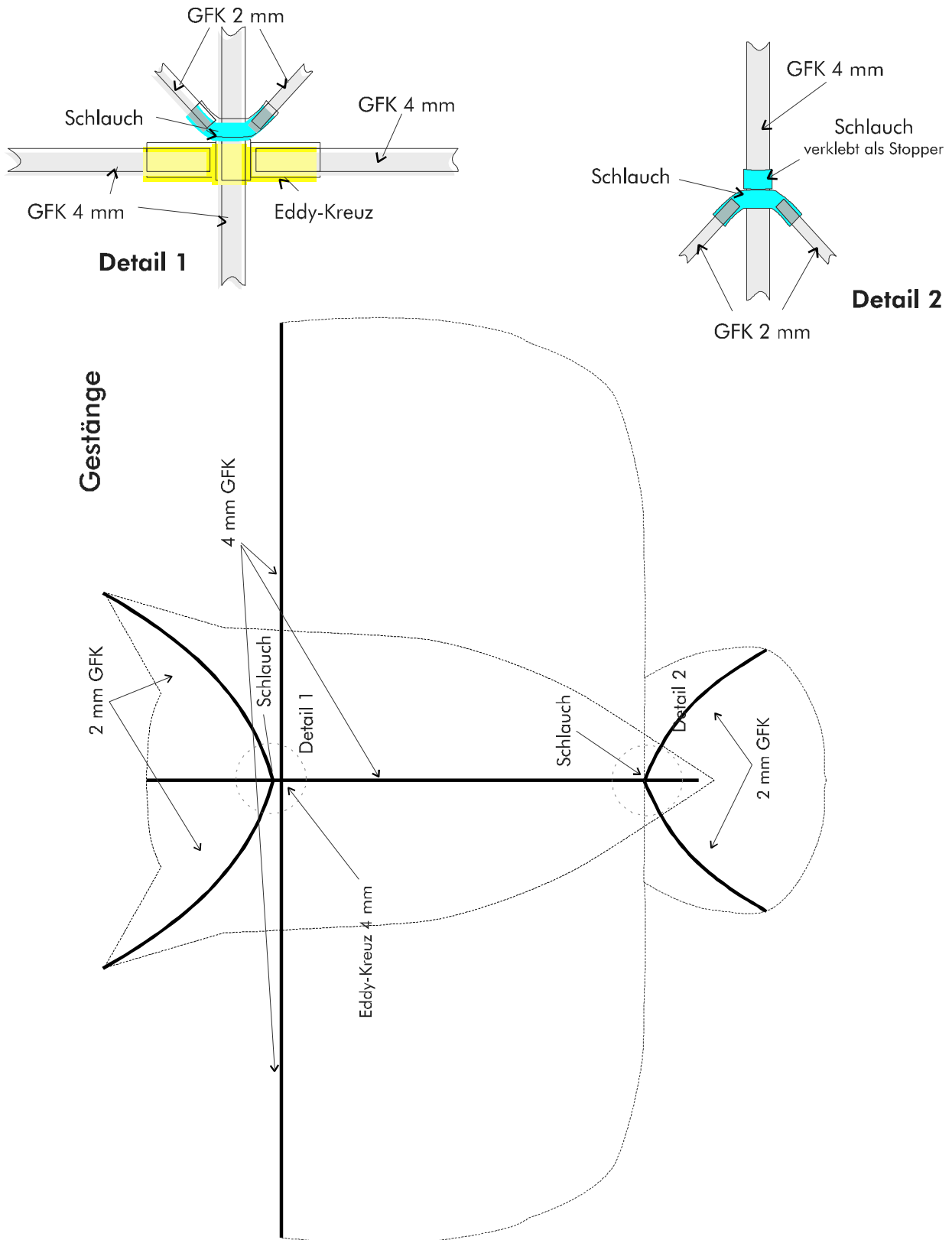
Abb. 3: Linkage dimensions and-details
