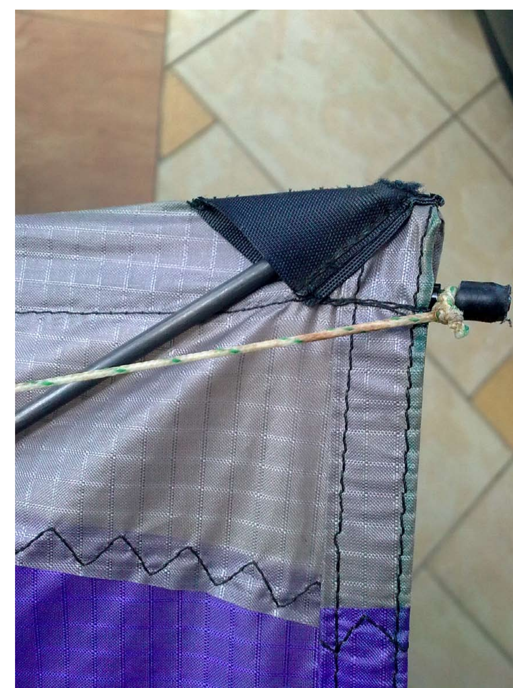
LE corner detail, LE Sleeve, LE spar corner stoppers & bowline tie
