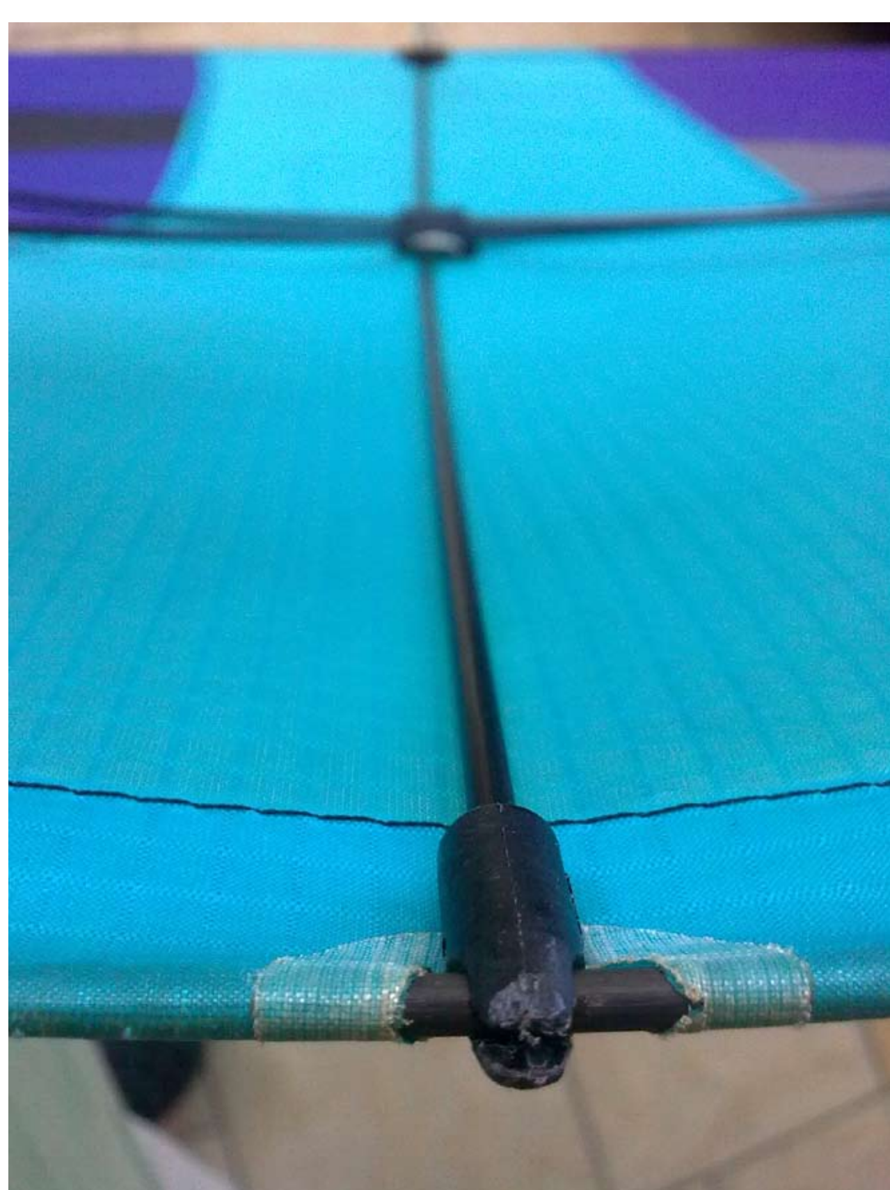
Spine detail, This part is LE looking down.
